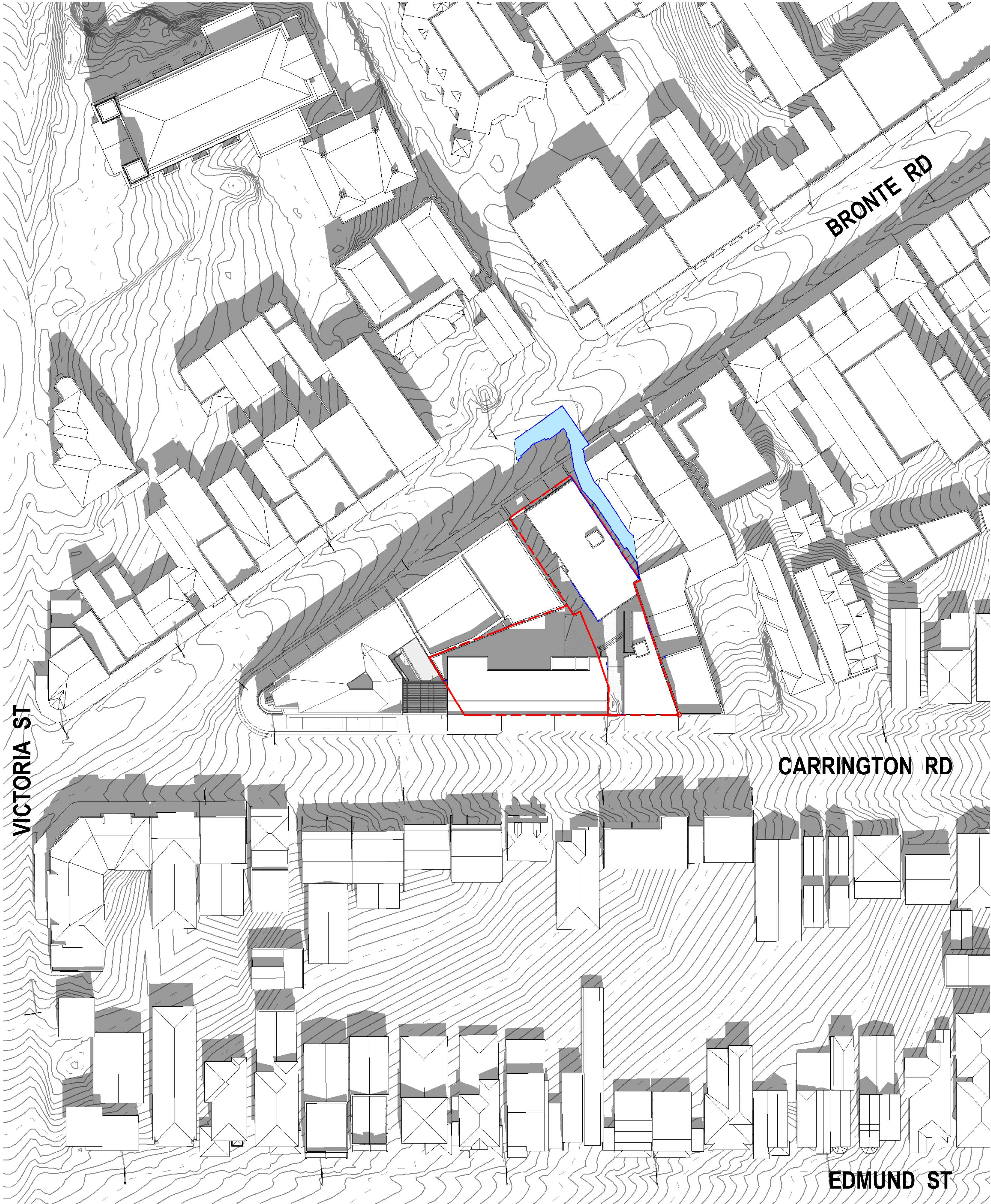
2 Shadow Plan - Proposed - Summer Solstice 3:00PM 1 : 500
